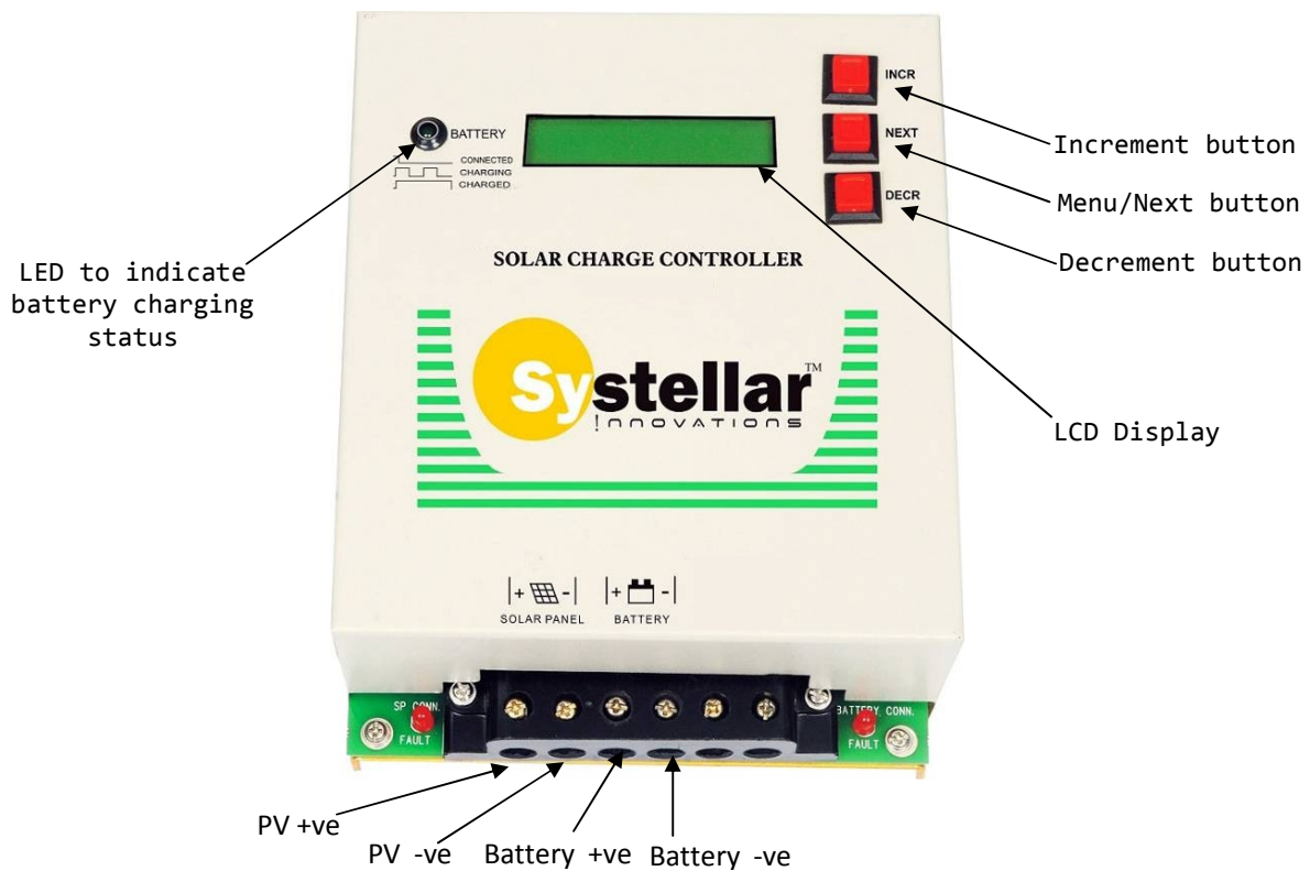
Front View
